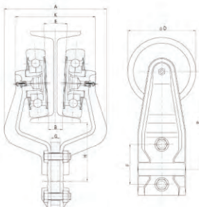
XT160 Trolley
