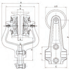
XT160 Trolley
